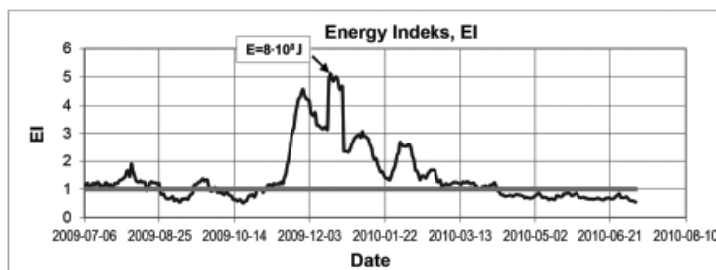
Fig. 2. An example of sequential distribution of EI parameter in moving time windows with the progress of 1 day in coal panel no. 3/503. On December 16, 2009 the strongest tremor of seismic energy E = 8 \cdot 10^8 \text{ J} ( M_L = 3.7 ) occurred at a time when was the highest value of EI parameter
